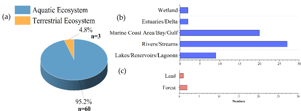
Figure 4. Summary of assessed ecosystems which adopted biological indicator method. The study was classified by aquatic ecosystem and terrestrial ecosystem (a). The aquatic ecosystem (b) and terrestrial ecosystem (c) were also classified.
