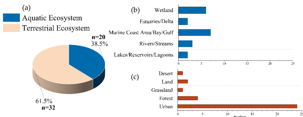
Figure 5. Summary of assessed ecosystems which adopted index system method. The study was classified by aquatic ecosystem and terrestrial ecosystem (a). The aquatic ecosystem (b) and terrestrial ecosystem (c) were also classified.
