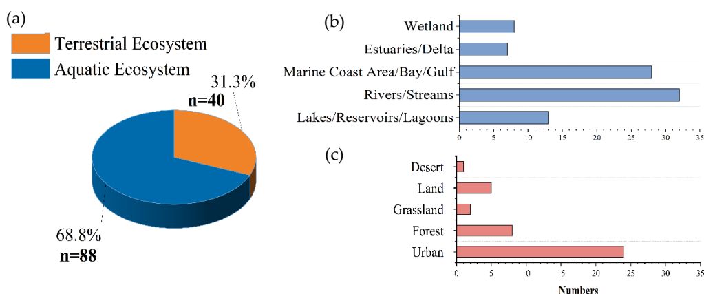
Figure 3. Summary of assessed ecosystem types in the publications found in the systematic review. All studies were classified by aquatic ecosystems and terrestrial ecosystem (a). The aquatic ecosystem (b) and terrestrial ecosystem (c) were also classified.
