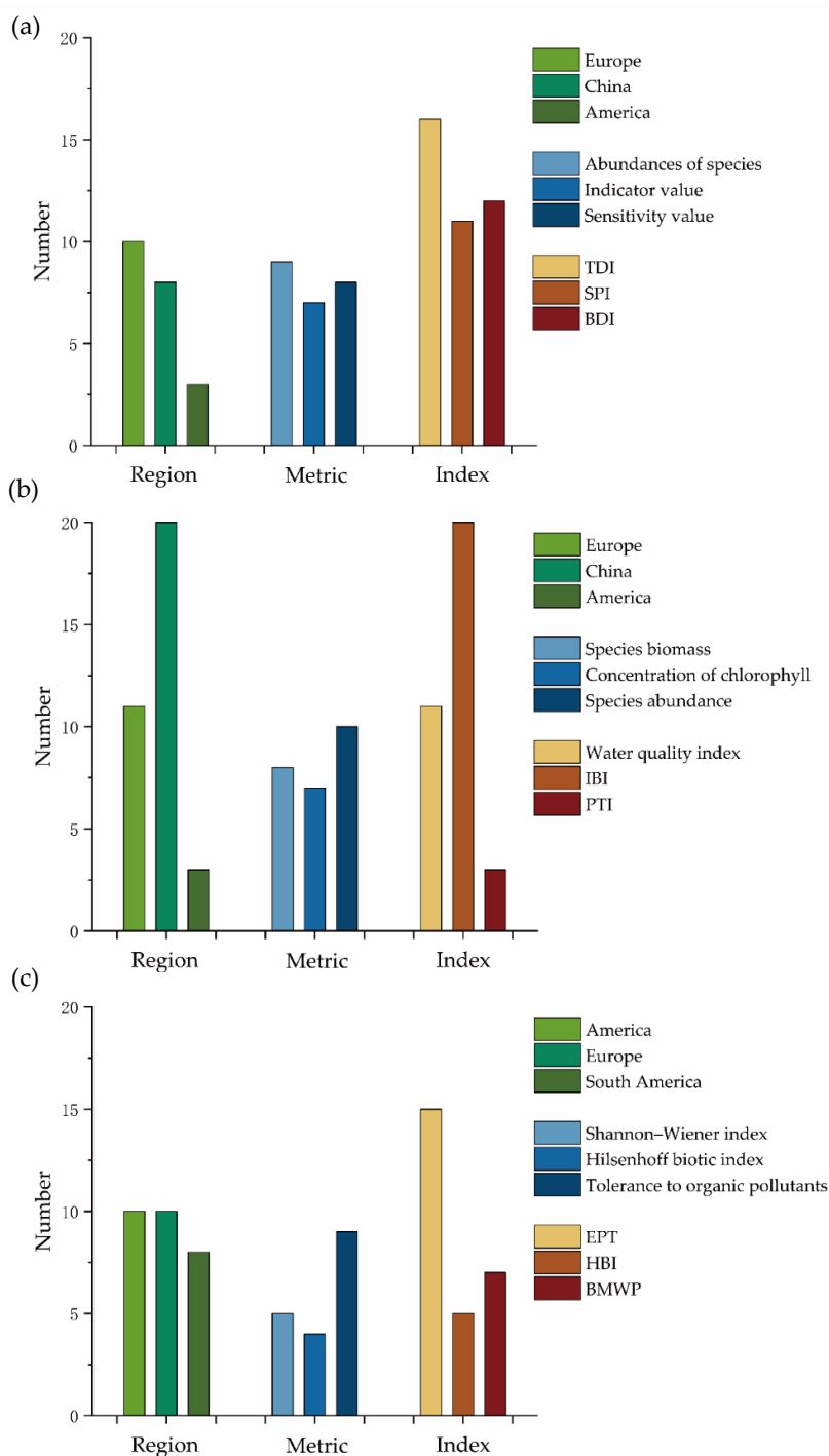
Figure 2. The most commonly used indices, metrics of indices, and where they are used most. (a) Diatom indices: BDI: Biological Diatom Index; SPI: Specific Pollution Sensitivity Index; TDI: Trophic Diatom Index. (b) Plankton indices: PTI: Phytoplankton Trophic Index; IBI: Index of Biotic Integrity. (c) Macroinvertebrate indices: BMWP: Biological Monitoring Working Party; HBI: Hilsenhoff biotic index; EPT: Ephemeroptera, Plecoptera, and Trichoptera.
