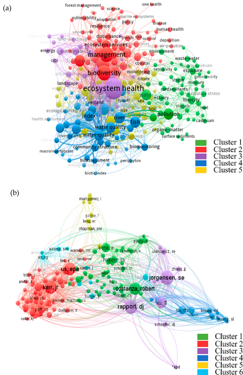
Figure 1. Bibliographic analysis results. (a) Keywords co-occurrence analysis. Cluster 1 is a toxicological cluster, clusters 2 and 5 are ecological clusters, cluster 3 and 4 are biological clusters. (b) Author co-citation analysis.
